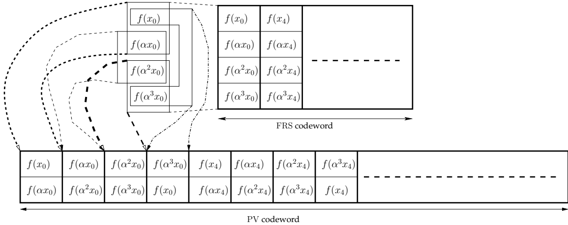
Figure 4: The correspondence between a folded Reed-Solomon code (with m = 4 ) evaluated over \{x_0, x_4, x_8, \dots, x_{n-4}\} and the Parvaresh Vardy code (of order s = 2 ) evaluated over \{x_0, x_1, x_2, \dots, x_{n-1}\} . Recall that by the choice of \alpha , x_{4i+j} = \alpha^j x_{4i} for 0 \leq i < n/4 and 0 < j \leq 3 ; \alpha^4 = 1 and f_1(X) = f(\alpha X) . The correspondence for the first block in the FRS codeword and the first four blocks in the PV codeword is shown explicitly in the left corner of the figure.
