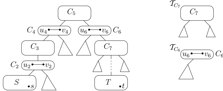
Figure 5: Partitioning of the PlaK 5 -component tree \mathcal{T}_G into pieces \mathcal{T}_{C_i} . The boxes indicate component nodes and the triangles indicate subtrees.
