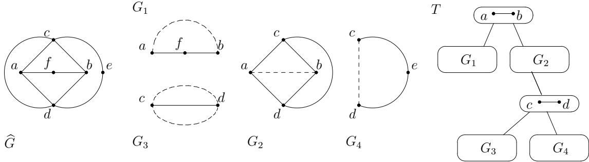
Figure 1: ([DLN + 08a]) The decomposition of a biconnected planar graph G . Its triconnected components are G_1, \dots, G_4 and the corresponding decomposition into the tree \mathcal{T} of triconnected components. The split pairs are (a, b) and (c, d) . Since the 3-connected separating pair (c, d) is connected by an edge in G , we also get \{c, d\} as triple-bond G_3 . The virtual edges corresponding to the 3-connected separating pairs are drawn with dashed lines.
