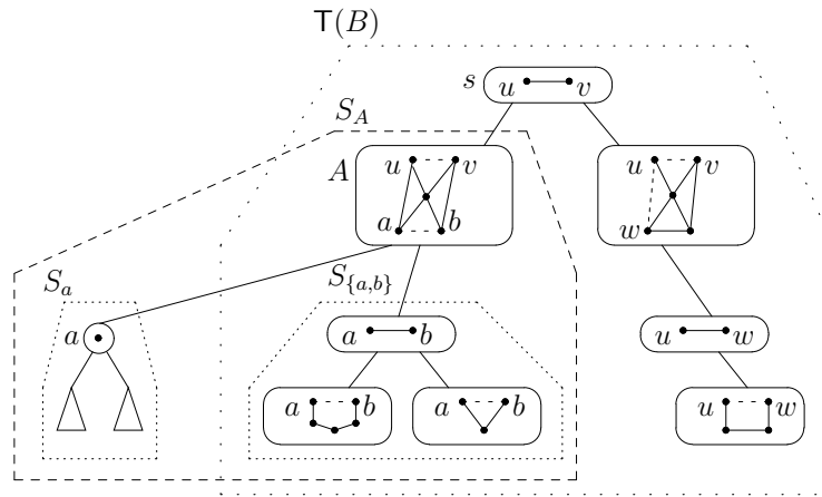
Figure 6: The triconnected component tree \mathbb{T}(B) of the biconnected component B . The triconnected component A contains the reference copy of articulation point a . If S_a is not a large child of B , then the subtree S_A consists of the subtree of \mathbb{T}(B) rooted at A and the subtree S_a . In contrast, S_a is not part of the subtree S_{\{a,b\}} because it does not contain the reference copy of a .
